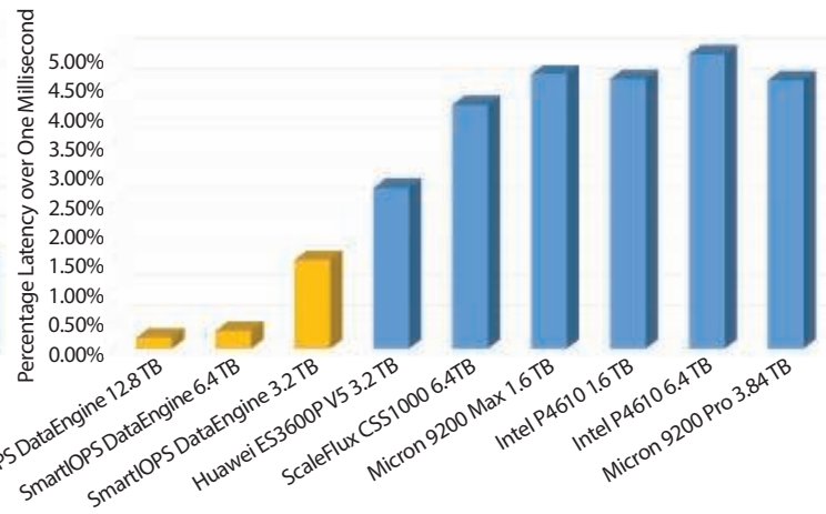
ACT Latency Results
